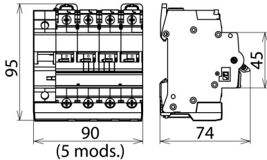
Dimension drawing POP 4 255 C40
