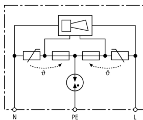
Basic circuit diagram STC 230
