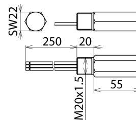
Dimension drawing DPI CD EXD 24 M
