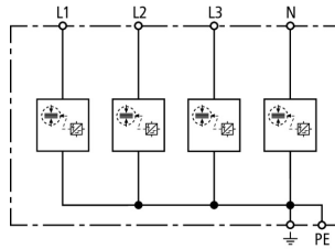
Basic circuit diagram DSH TNS 255
