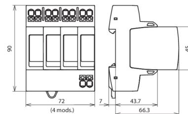
Dimension drawing DG MP TNS 275
