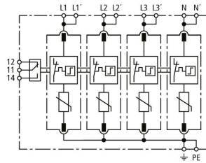
Basic circuit diagram DG MP TNS 275 FM
