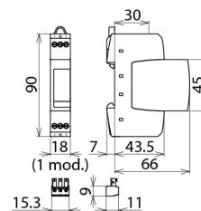
Dimension drawing DR M 2P 255 FM
