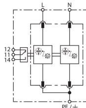
Basic circuit diagram DV M2 TN 255 FM
