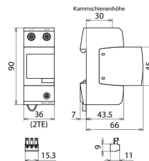
Dimension drawing DV M2 TN 255 FM
