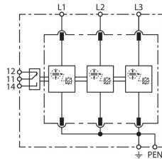
Basic circuit diagram DV M2 TNC 255 FM
